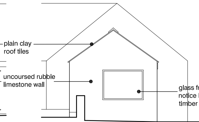
elevation - south/east
